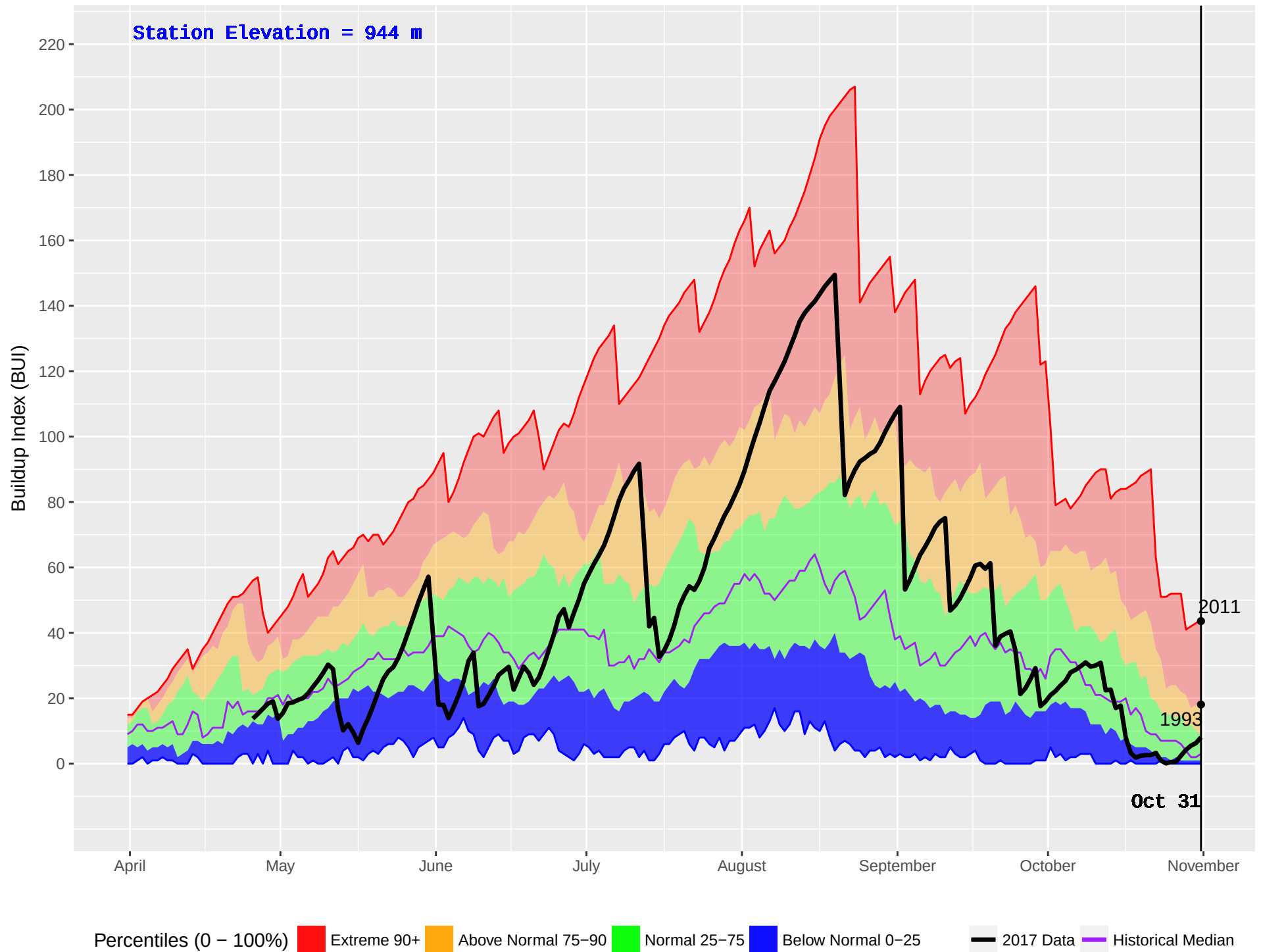
GRASSY PLAINS HUB (161) : Historical (1970–2016) and Current (2017) Noon Buildup Index (BUI)
