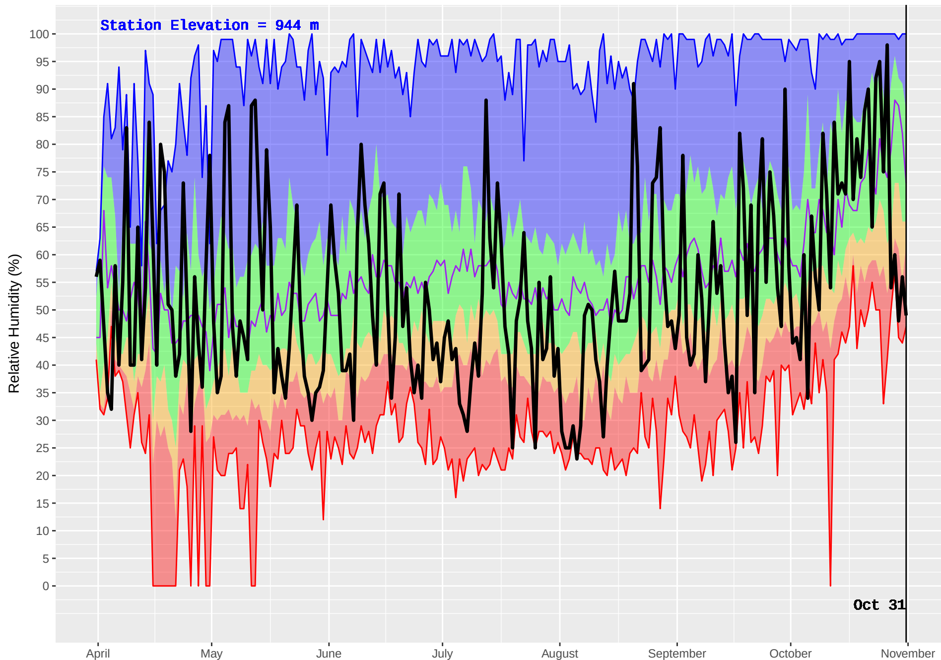
GRASSY PLAINS HUB (161) : Historical (1970–2016) and Current (2017) Noon Relative Humidity
